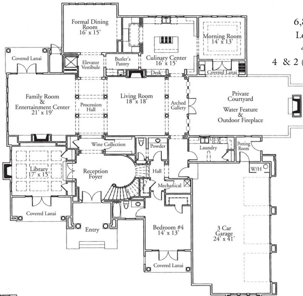
First Floor Plan Living Area 3,810 sf
